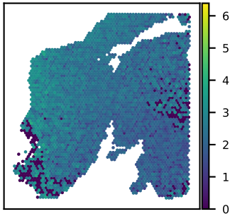
SNU24A CLDND1 expression Moran's I = 0.29
