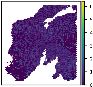
SNU24A STRBP expression Moran's I = 0.05
