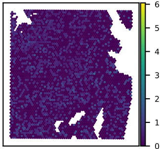
SNU51A DCPS expression Moran's I = 0.02
