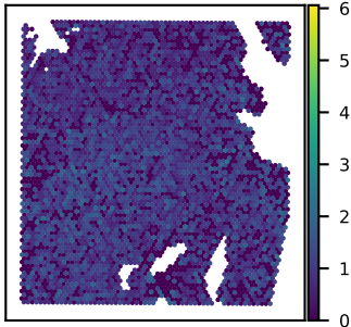
SNU51A PNMA8C expression Moran's I = 0.07
