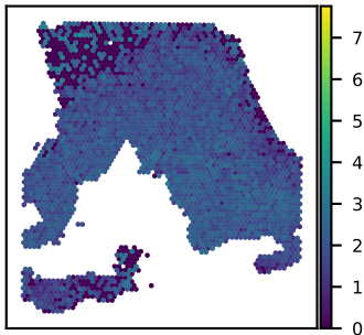
SNU18A KCTD12 expression Moran's I = 0.29
