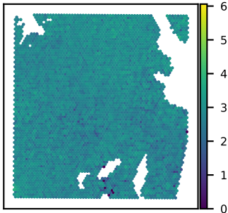
SNU51A DPYSL2 expression Moran's I = 0.20
