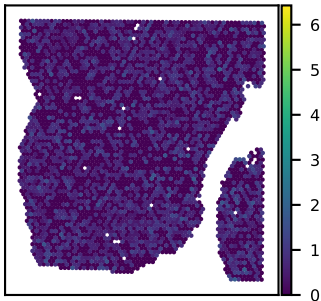
SNU25B CLEC16A expression Moran's I = 0.01
