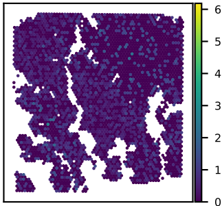
SNU16B PLEKHM1 expression Moran's I = 0.01
