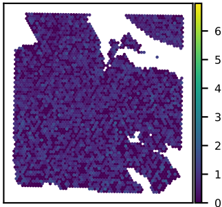
SNU24B TOR1AIP1 expression Moran's I = 0.01
