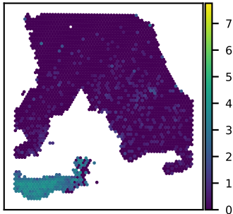
SNU18A SNAP25 expression Moran's I = 0.82
