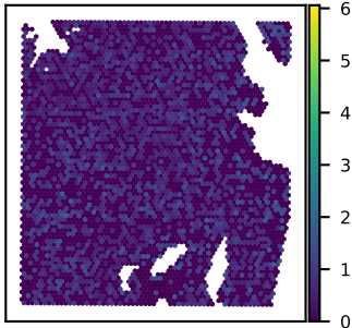
SNU51A EVI5L expression Moran's I = 0.01
