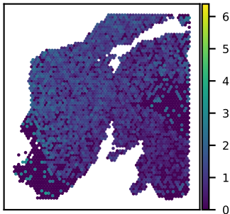
SNU24A CNTN2 expression Moran's I = 0.23
