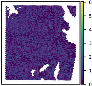
SNU51A CNOT1 expression Moran's I = 0.02
