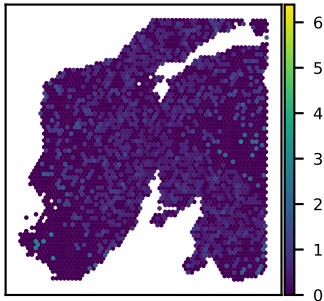
SNU24A C2orf42 expression Moran's I = 0.03
