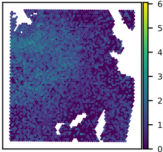
SNU51A PDGFRA expression Moran's I = 0.42
