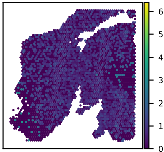
SNU24A FBXO38 expression Moran's I = 0.03
