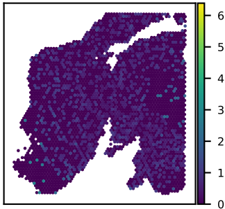
SNU24A SCAI expression Moran's I = 0.02
