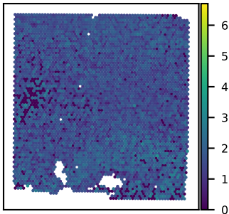
SNU43A CTXN1 expression Moran's I = 0.08
