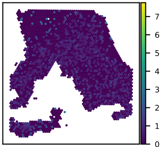
SNU18A PACRGL expression Moran's I = 0.04
