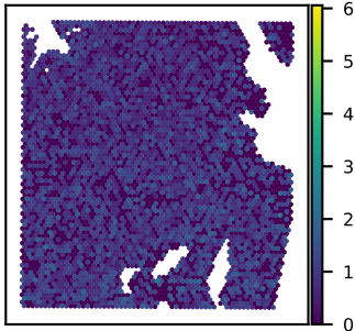
SNU51A MLLT1 expression Moran's I = 0.03
