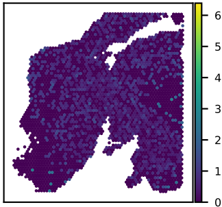
SNU24A CITED4 expression Moran's I = 0.05
