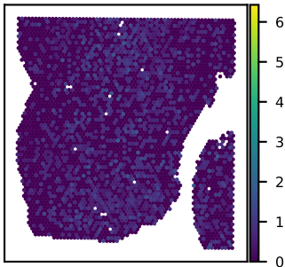
SNU25B DLGAP3 expression Moran's I = 0.05
