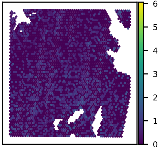
SNU51A RIMKLA expression Moran's I = 0.03
