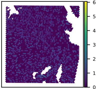
SNU51A ZSCAN30 expression Moran's I = 0.01
