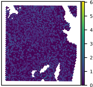
SNU51A RRAGD expression Moran's I = 0.02
