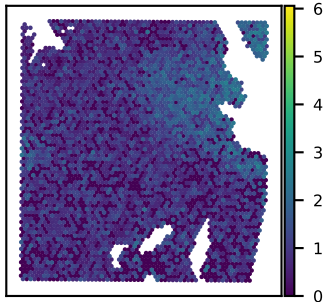
SNU51A BSCL2 expression Moran's I = 0.28
