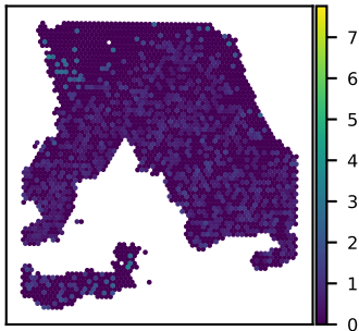
SNU18A CEP57L1 expression Moran's I = 0.02
