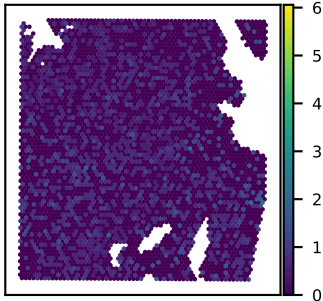
SNU51A CNOT6 expression Moran's I = 0.02
