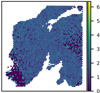
SNU24A PDCD6 expression Moran's I = 0.17
