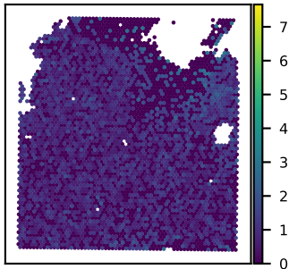
SNU21B NOP58 expression Moran's I = 0.07
