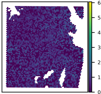
SNU51A TMEM132A expression Moran's I = 0.03
