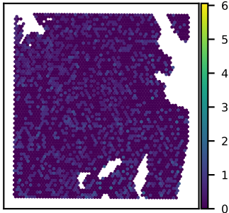
SNU51A DHDDS expression Moran's I = 0.02
