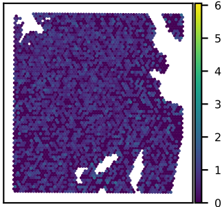
SNU51A EIF5B expression Moran's I = 0.02
