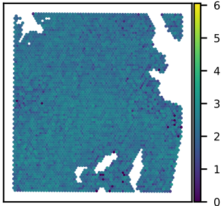
SNU51A PARK7 expression Moran's I = 0.09
