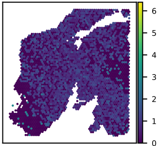
SNU24A ZDHHC5 expression Moran's I = 0.10
