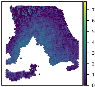
SNU18A DBNDD2 expression Moran's I = 0.50
