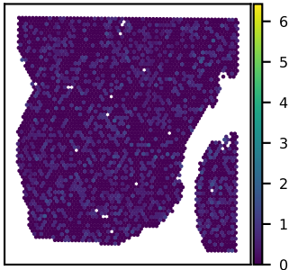
SNU25B SLC16A2 expression Moran's I = 0.01
