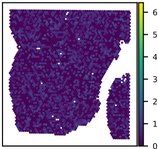
SNU25B PACRGL expression Moran's I = 0.01
