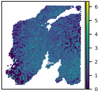
SNU24A SERPINE1 expression Moran's I = 0.28
