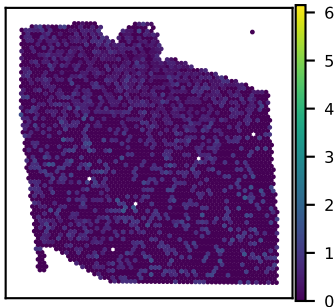
SNU27A SLC35A2 expression Moran's I = 0.01
