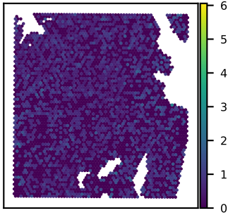
SNU51A RAB1B expression Moran's I = 0.01
