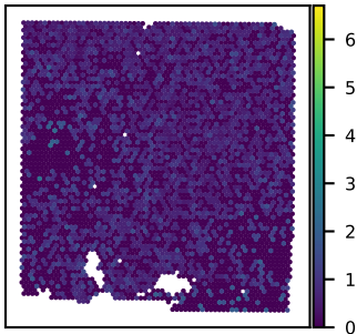
SNU43A SMARCD2 expression Moran's I = 0.03
