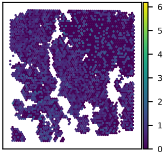
SNU16B TOR1AIP1 expression Moran's I = 0.03
