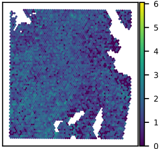
SNU51A CCN2 expression Moran's I = 0.20
