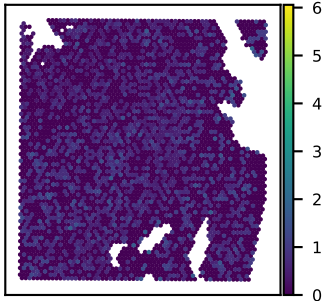
SNU51A STRBP expression Moran's I = 0.01
