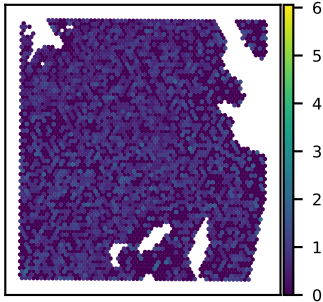
SNU51A SLC12A9 expression Moran's I = 0.01
