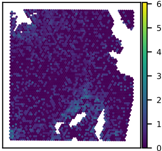
SNU51A SPNS2 expression Moran's I = 0.22
