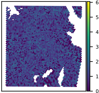
SNU51A DENND5A expression Moran's I = 0.03
