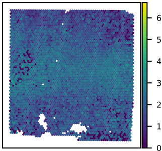
SNU43A HIST1H4A expression Moran's I = 0.35
