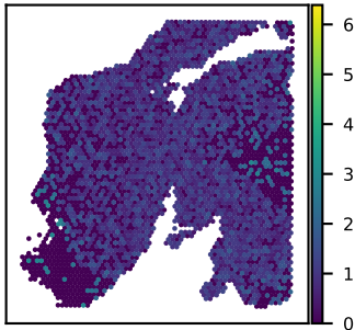
SNU24A IFT46 expression Moran's I = 0.06
